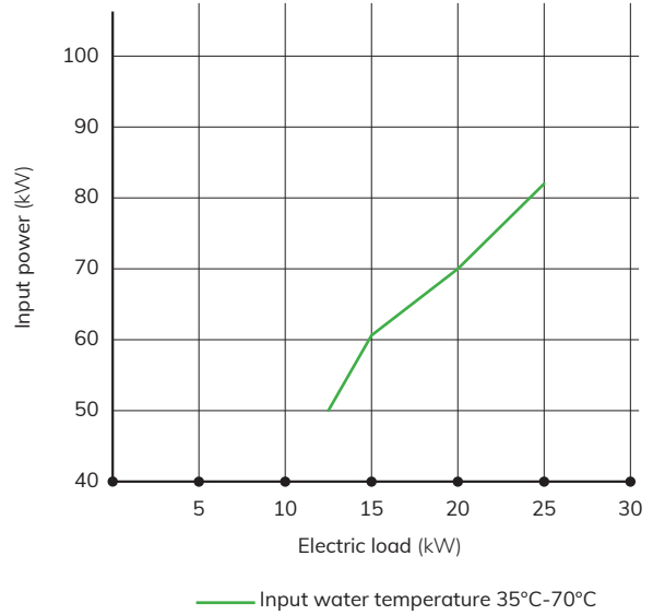
Input power vs electric load
